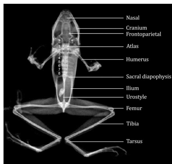
Figure 3. Osteology of an adult Bijurana nicobariensis comb. nov. (DOSMB 05050) from Little Nicobar, India.
