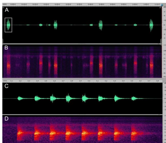
Figure 8. The call of Bijurana nicobariensis comb. nov. (A) Oscillogram and (B) spectrogram; (C & D) magnified view of a single note composed of eight pulses.
